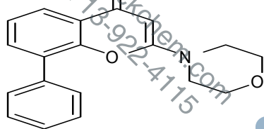
S110502, DMSO-d6
