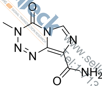
S123702, DMSO-d6
