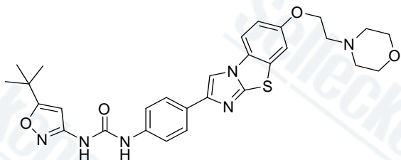
S152601, DMSO-d6
