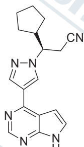
S137815, DMSO-d6
